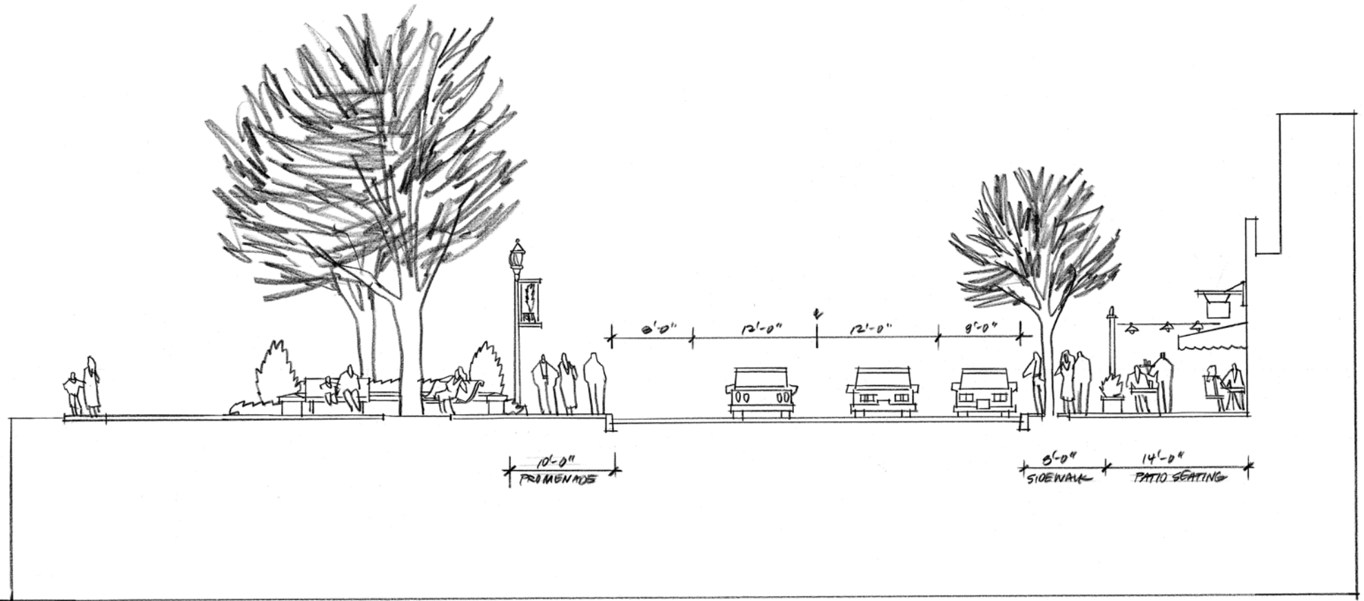
SECTION ELEVATION @ CORNER ENTRY TO ROSS COMMON SCALE = 1" = 4'
